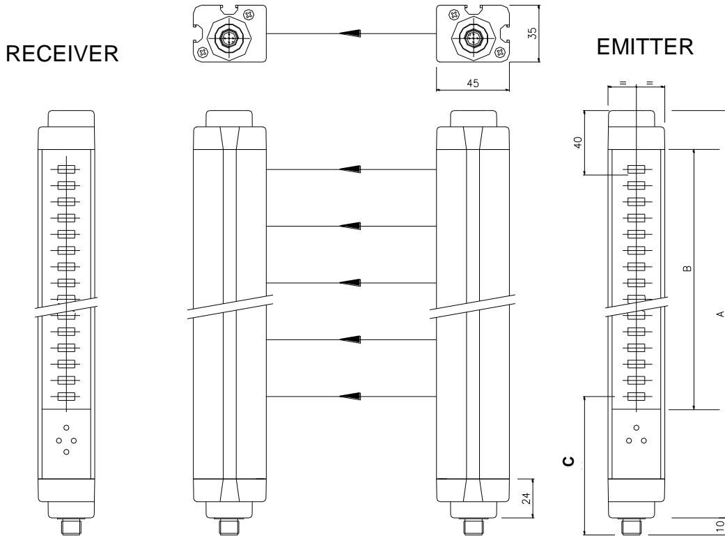
Figure 19 Emitter and Receiver
